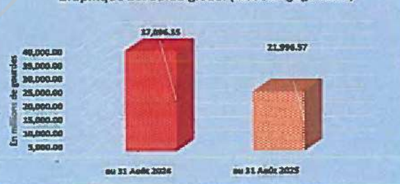
Graphique 10. Solde global ( base engagement)
